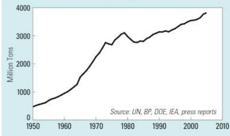
Figure 1. World Oil Consumption, 1950–2005
