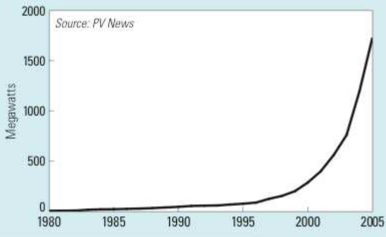
Figure 1. World Annual Photovoltaic Production, 1980–2005
