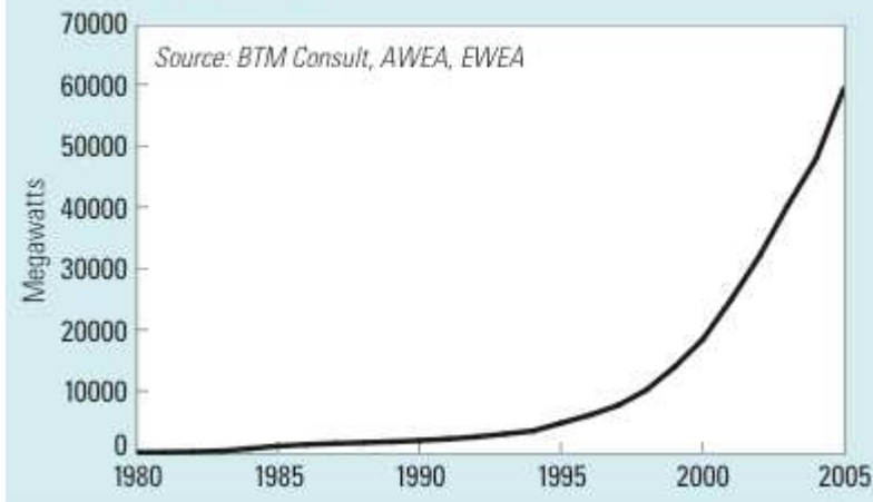
Figure 1. World Wind Energy Generating Capacity, 1980–2005
