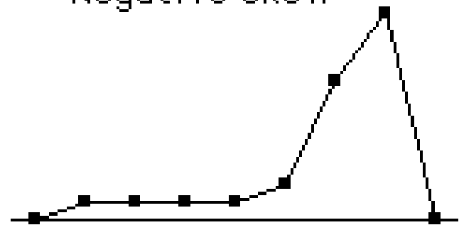
Negative skew
