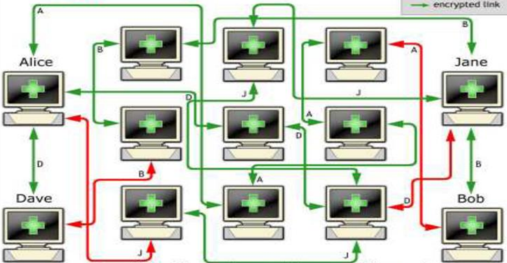
Nine Tor nodes and 4 users / Tor nodes
