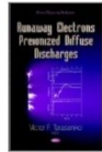
Runaway Electrons Preionized Diffuse Discharges by Tarasenko, V. F.
