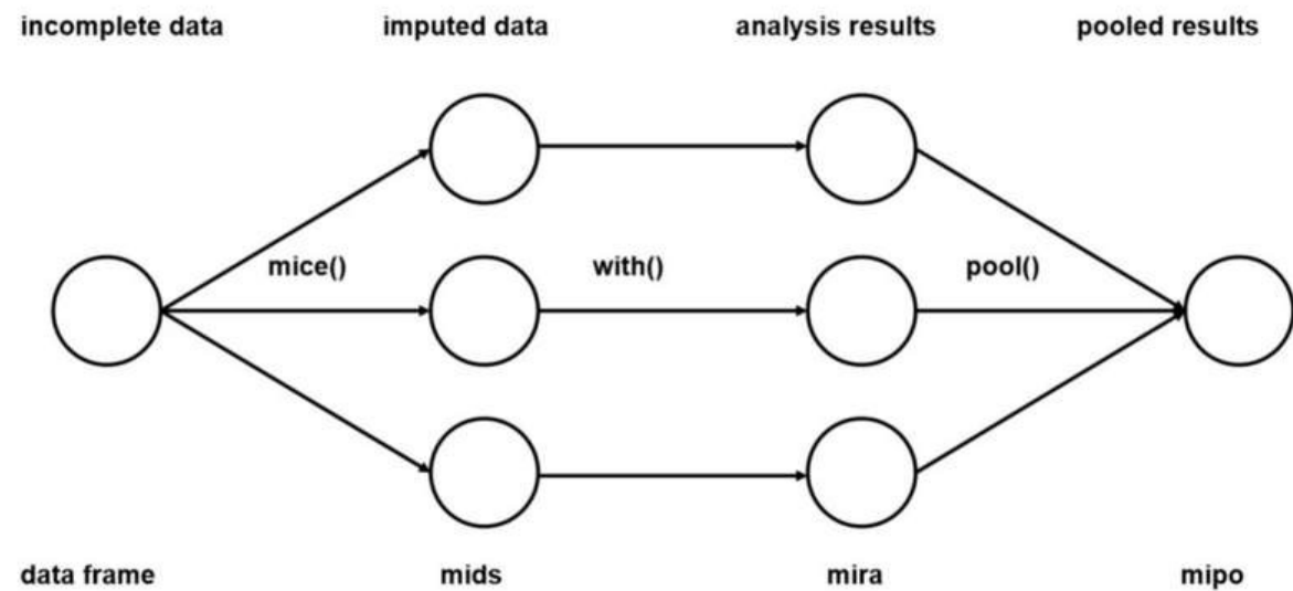
Figure 1: Main steps used in multiple imputation.
