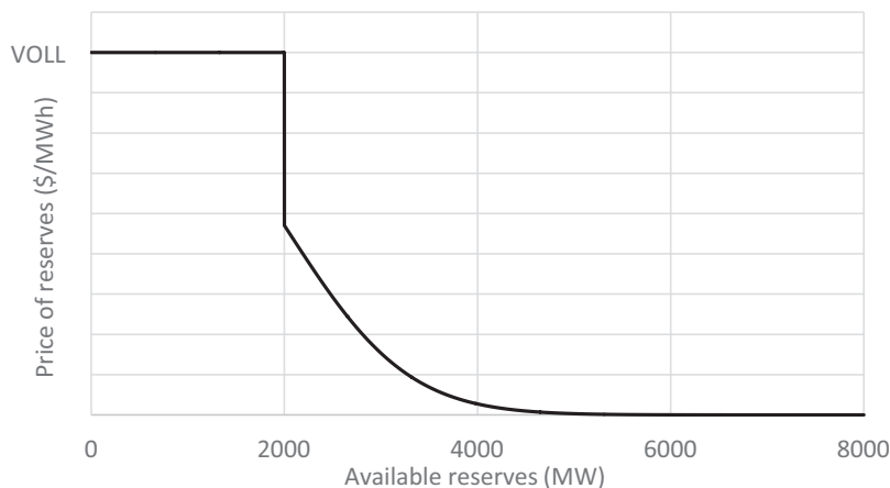
Figure 1: ERCOT's operating reserve demand curve
