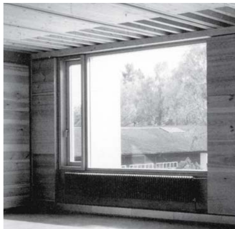
Fig. 280: Window The window is fitted directly into the structural frame. A narrow opening light for ventilation has been included instead of just providing a large undivided glazed area.
