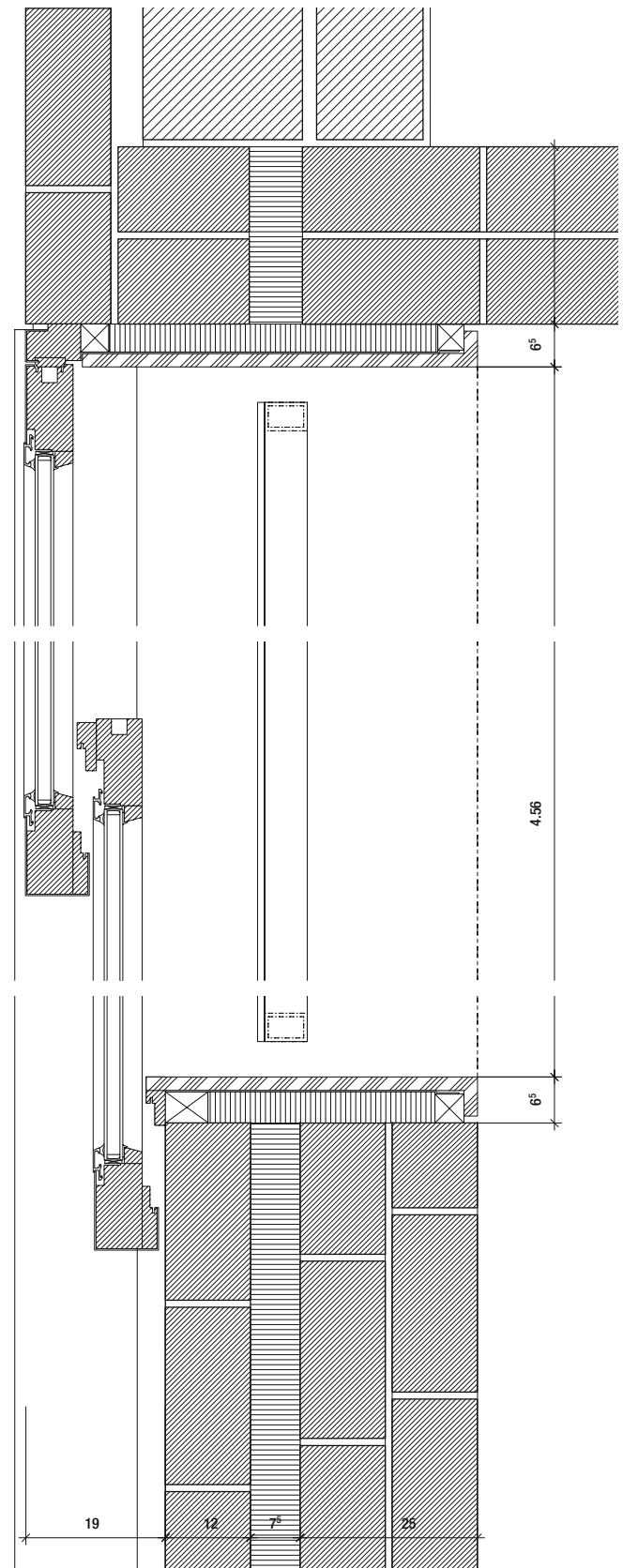
Fig. 64: Plan, 1:10 The windows are fitted without a true rectangular frame.
