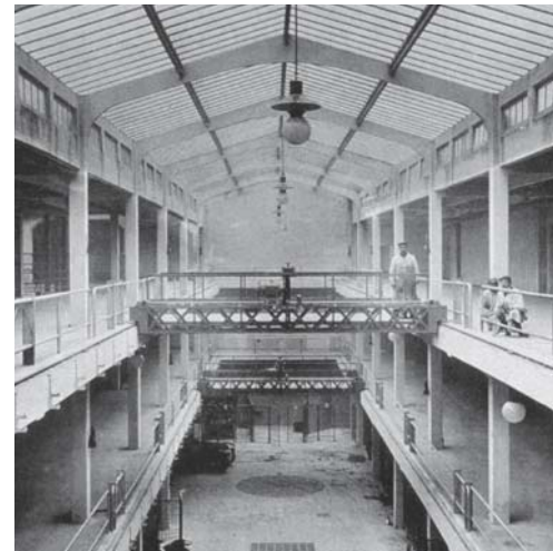
Abb. 57: Fixed-based portal frame Auguste + Gustave Perret: Ponthieu garage, Paris (F), 1906
