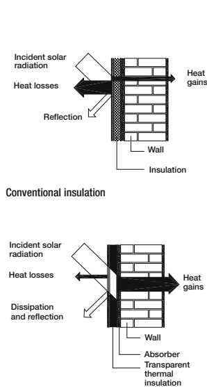
Fig. 8: Transparent thermal insulation
