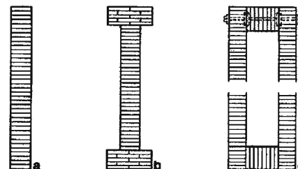
Fig. 15: Cross-sections in glued laminated timber a Rectangular b I-section c Box section, doweled or glued
