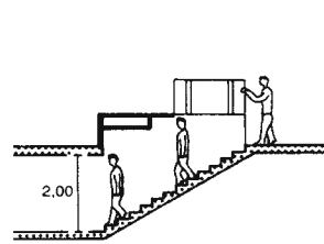
9 Basement entrances and trapdoors should be avoided; however, the above combination is advantageous and presents no risks.
