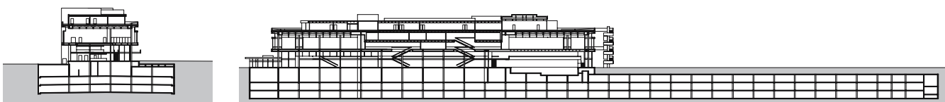
Fig. 3: The internal layouts of substructure and superstructure have developed independently of each other but still use a common column grid. Roland Rohn: Hoffmann-La Roche staff accommodation, Basel (CH), 1971
