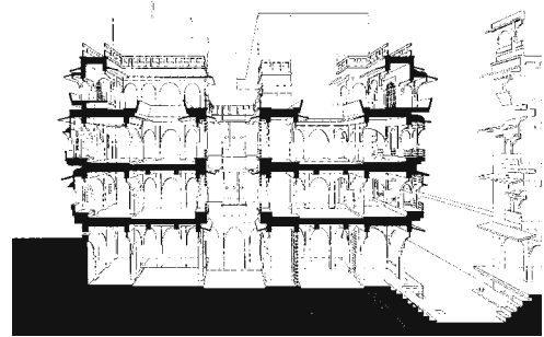
Fig. 34: Exploiting the stack effect: fresh air flows through the open ground floor and rises in the internal courtyard. House, Jaisalmer (India), 15th century
