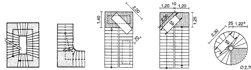
18 Diagonal first step and distorted steps save space 19 Curving the steps in narrow stair shafts saves on landing width 20 Minimum space requirement for transporting furniture 21 Space requirement for stretcher 22 Spiral stairs: space requirement for stretcher
