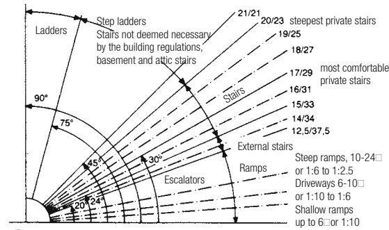
1 Pitches for ramps, external stairs, private stairs, plant access stairs and ladders
