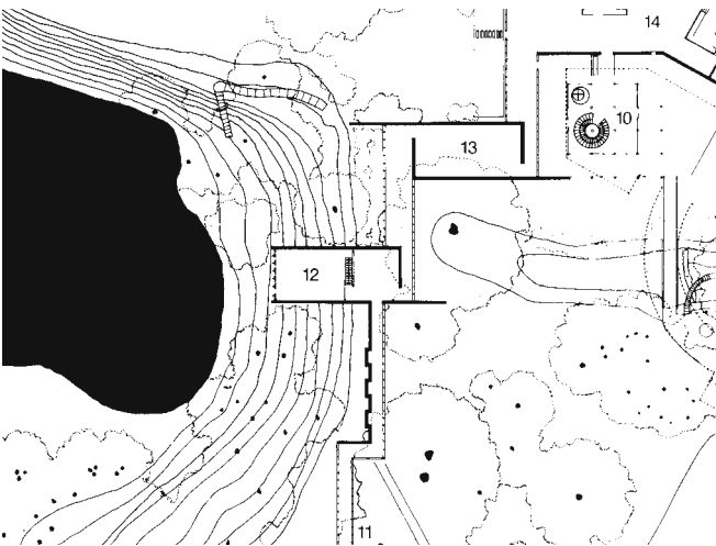
Fig. 47: Nature almost within reach thanks to the omission of spandrel panel and lintel Bo + Wohlert: Louisiana Museum, Humlebaek (DK), 1958
