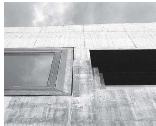
Fig. 152: Contrast between inward- and outward-opening windows
