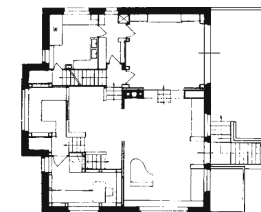
Fig. 92: Section, plan of 1st floor Adolf Loos: Möller House, Vienna (A), 1928
