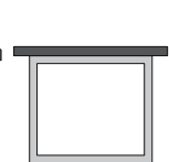
Fig. 43: Warm deck flat roof no air cavity
