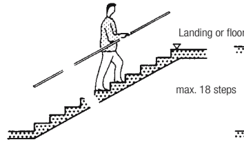
5 Standard stairs 17/29, max. 18 steps
