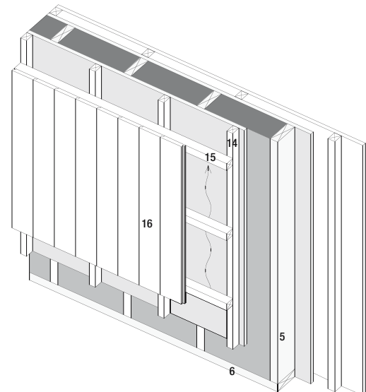
Axonometric view of layers Horizontal sheathing (top) and vertical sheathing (bottom)
