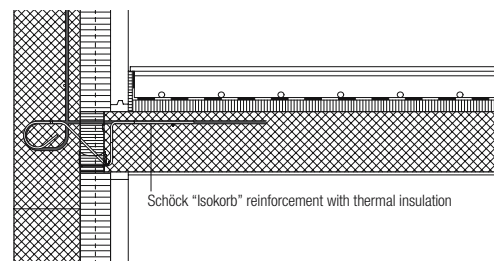
Fig. 38: Construction detail
