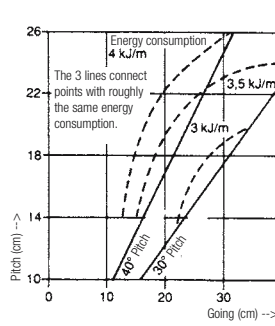
4 Energy consumption for an adult climbing a flight of stairs
