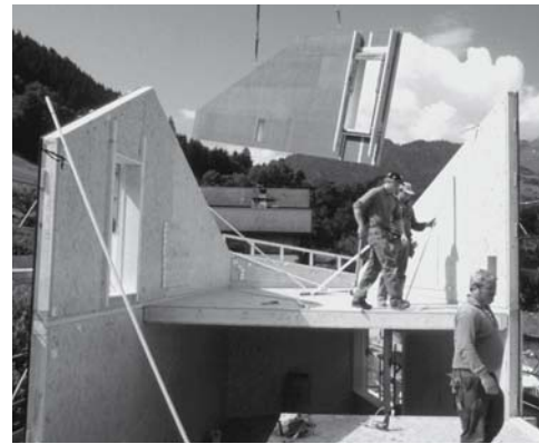
Fig. 47: Erection of platform frame elements with sheathing both sides Beার্থ & Deplazes: private house (Willimann), Sevgelin (CH), 1998
