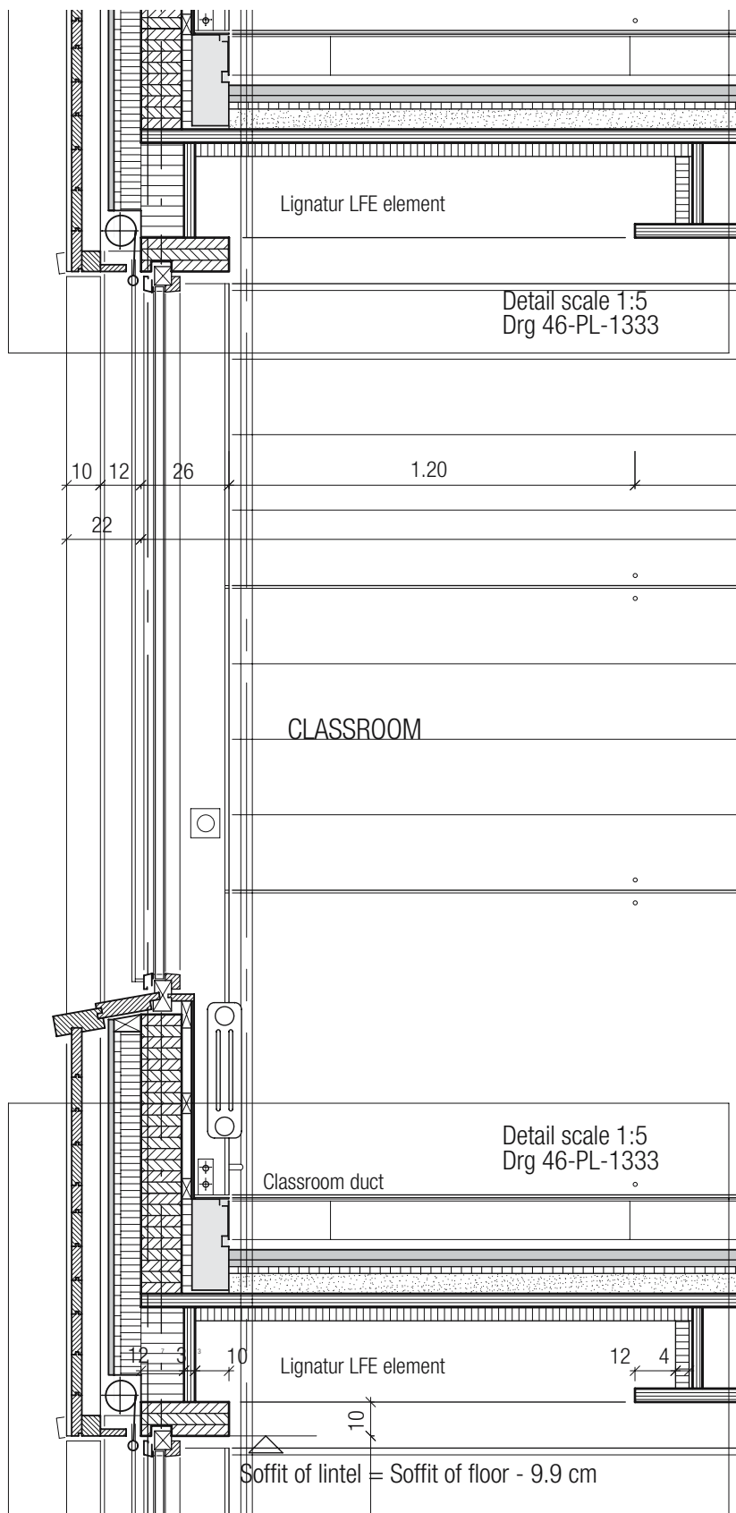
Fig. 279: Window detail, 1:20
