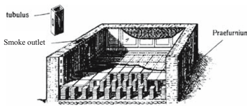
Fig. 90: Isometric view of hypocaust ( hypocaust = heating from below)
