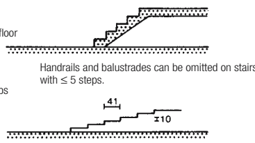
6 Stairs without handrail(s)
