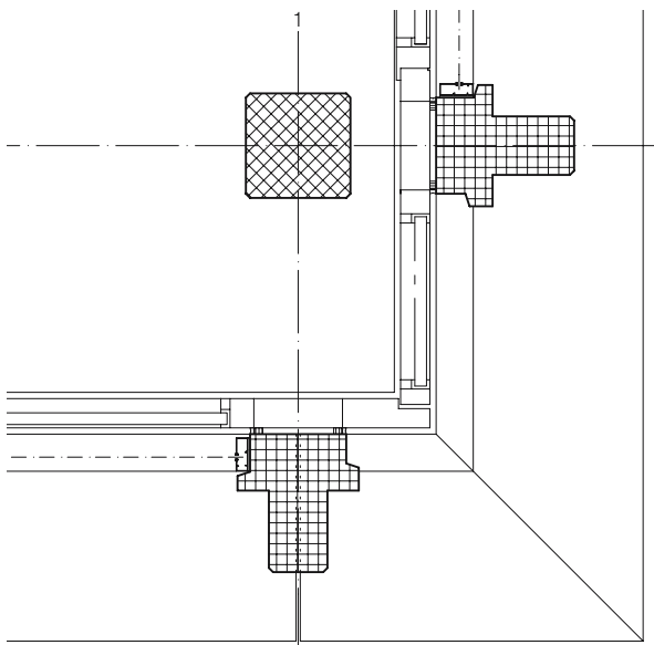
Fig. 228: Detail, 1:20 Non-symmetrical corner at ground floor level showing plinth element
