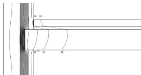
Fig. 35: Isotherms diagram
