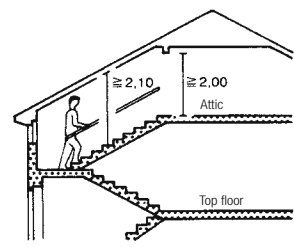
8 If rafters and beams run in the same direction as the stair flight, it is possible to save space and expensive trimmers.
