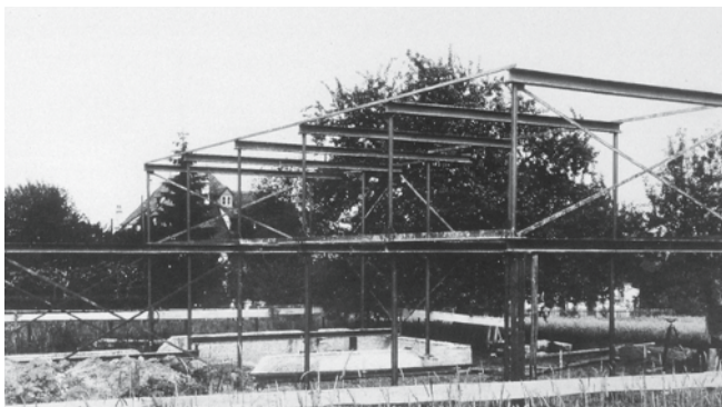
Fig. 112: The primary loadbearing structure is a horizontal and vertical succession of separate yokes. Artaria & Schmidt: Schaeffer House, Riehen (CH), 1927–28
