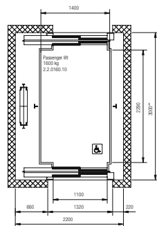
Passenger and goods lift, large, doors on two sides
