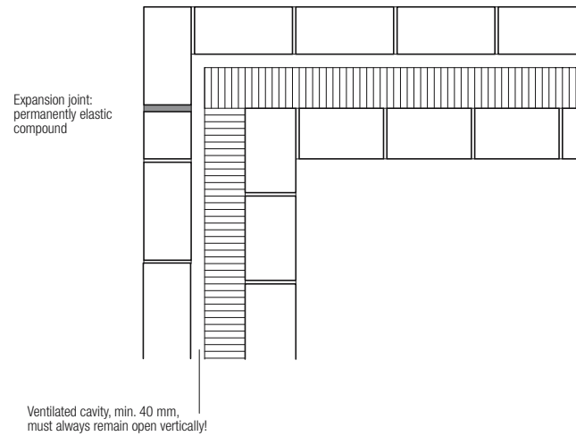
Plan, course 2
