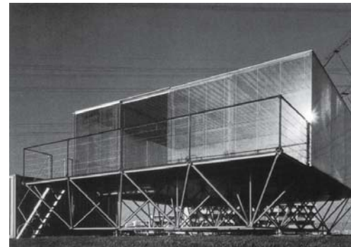
Fig. 70: The space frame distributes the loads of the building to four pad foundations. Bentham Crouwel: private house, Almere (NL), 1984
