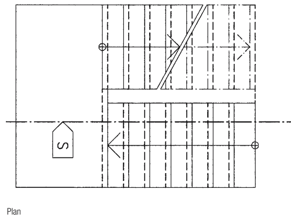
Fig. 17: Dog-leg stairs Plan and section
