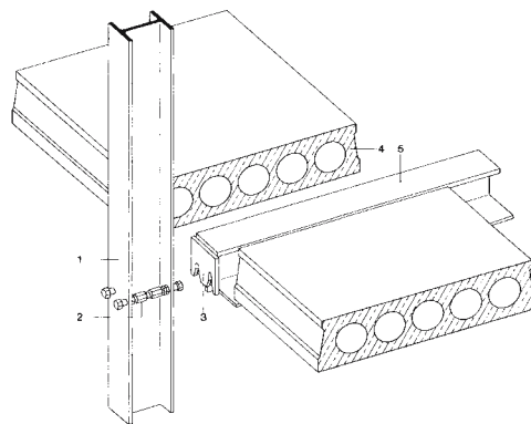
Fig. 50: Prestressed hollow-core planks
