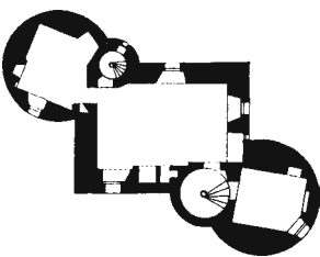
Fig. 84: Claypott Castle
