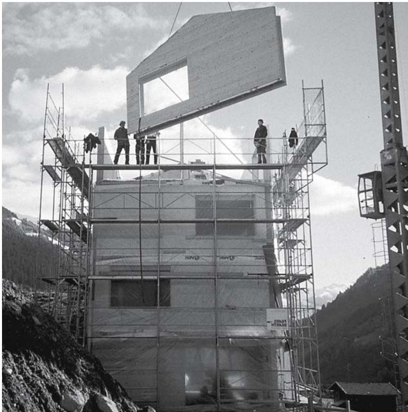
Fig. 2: Solid timber panel building during construction Bearth & Deplazes: private house (Bearth-Candinas), Sumvitg (CH), 1998
