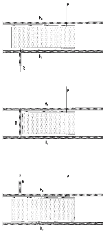
Fig. 169: Shear wall schemes Shear wall as unyielding structural element with single discrete support. The rotational effect of load P and support reaction R is eliminated by the horizontal couple H_0 and H_u generated in the floor slabs.
