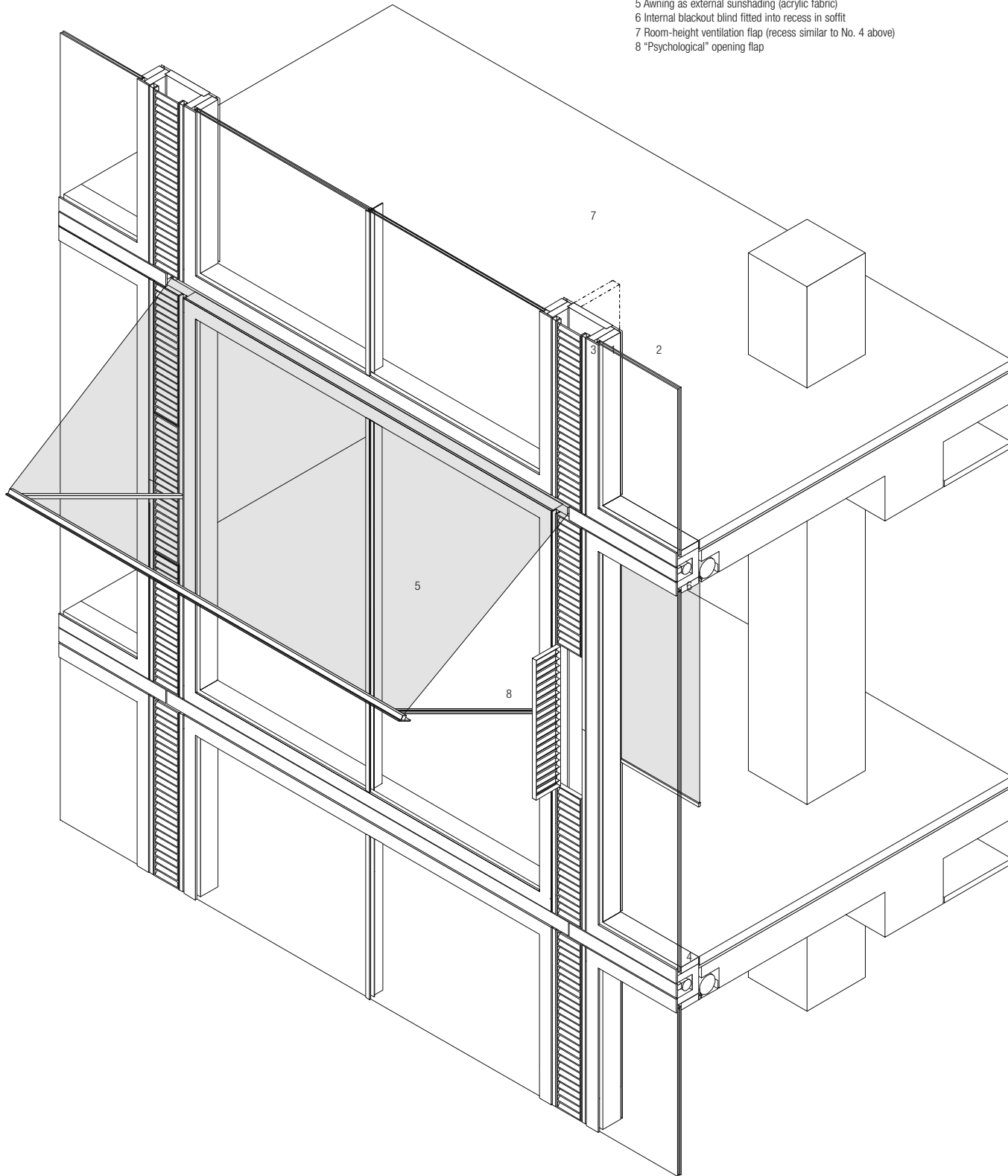
Fig. 247: Facade details
