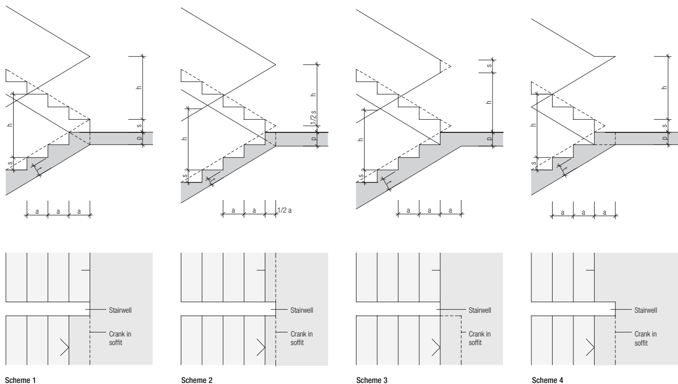
Fig. 22: Schemes (above)
