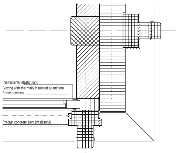
Fig. 227: Detail, 1:20 Corner showing junction of masonry infill and external thermal insulation, rendered
