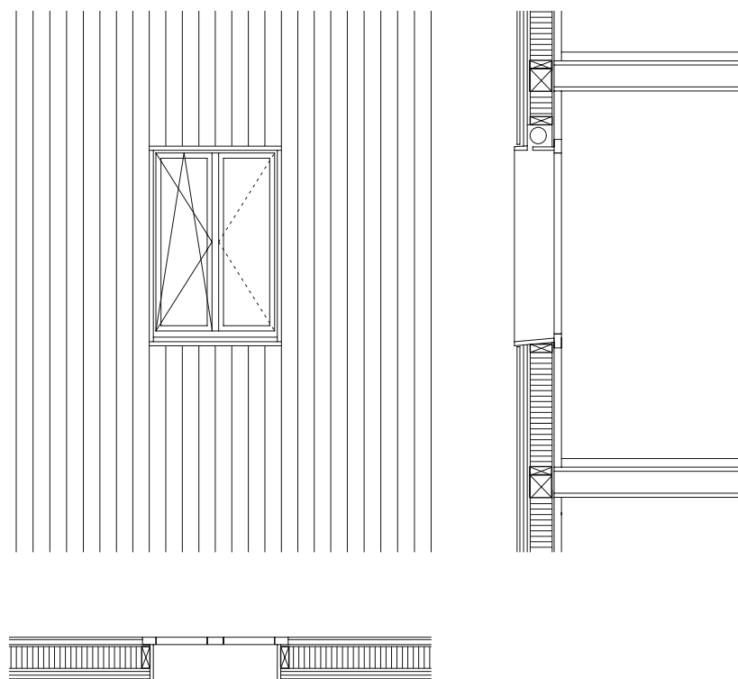
Plan, section, elevation, scale 1:50
