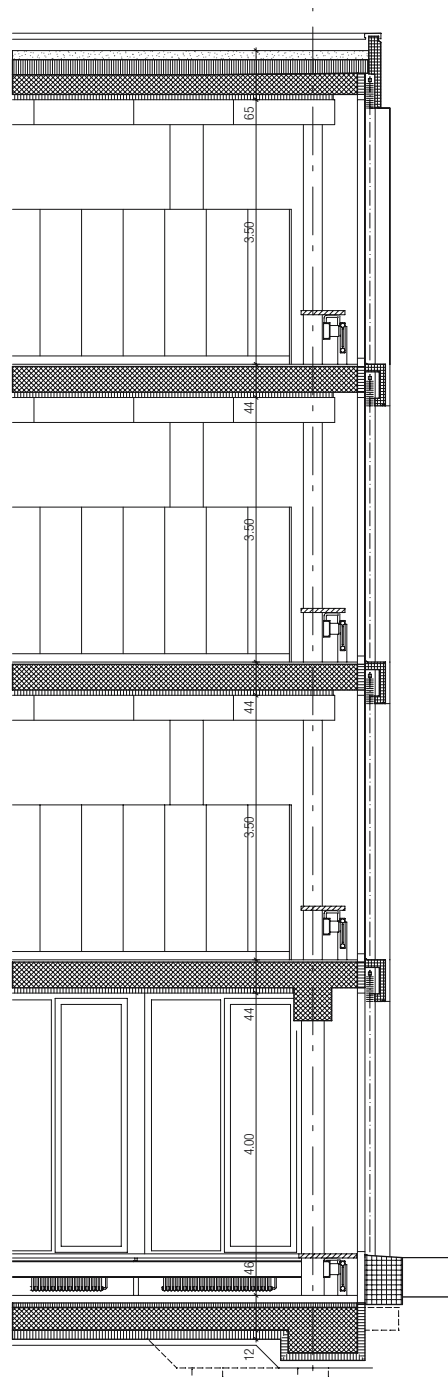
Fig. 221: Section, 1:50
