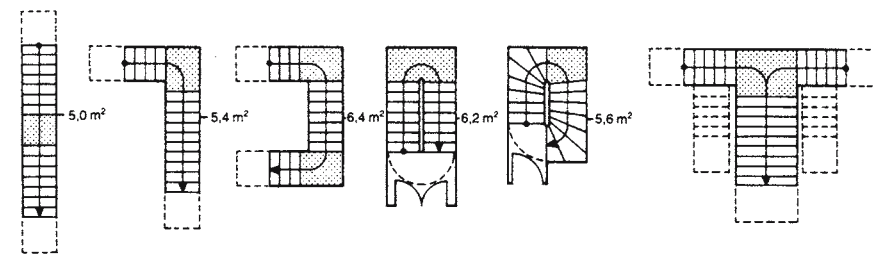
12-16 Stairs with landings cover the plan area of a single flight + landing area - 1 tread area. Stairs with landings are necessary for storey heights 2.75 m. Landing width stair width. 17 Stair with three flights: expensive, impractical, wastes space
