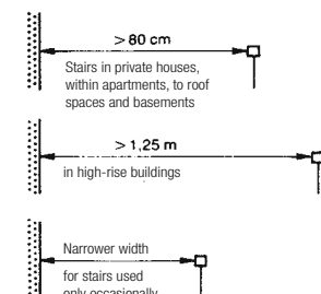
15 Measuring the usable stair width
