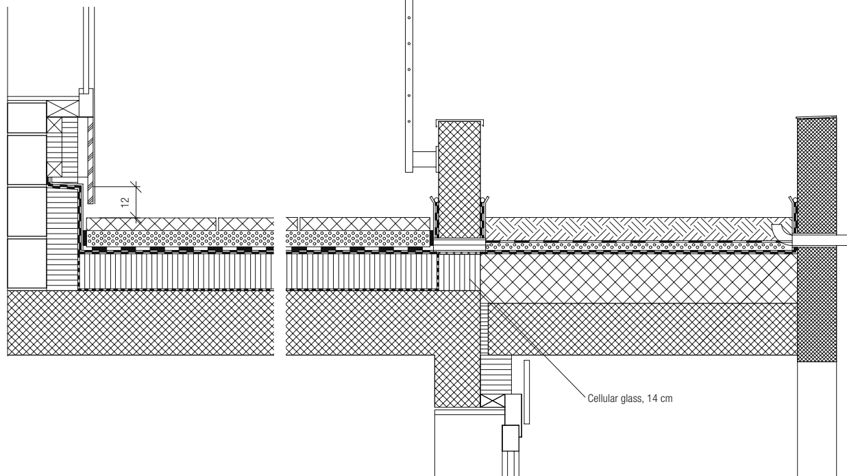
Warm deck, suitable for foot traffic, terrace
