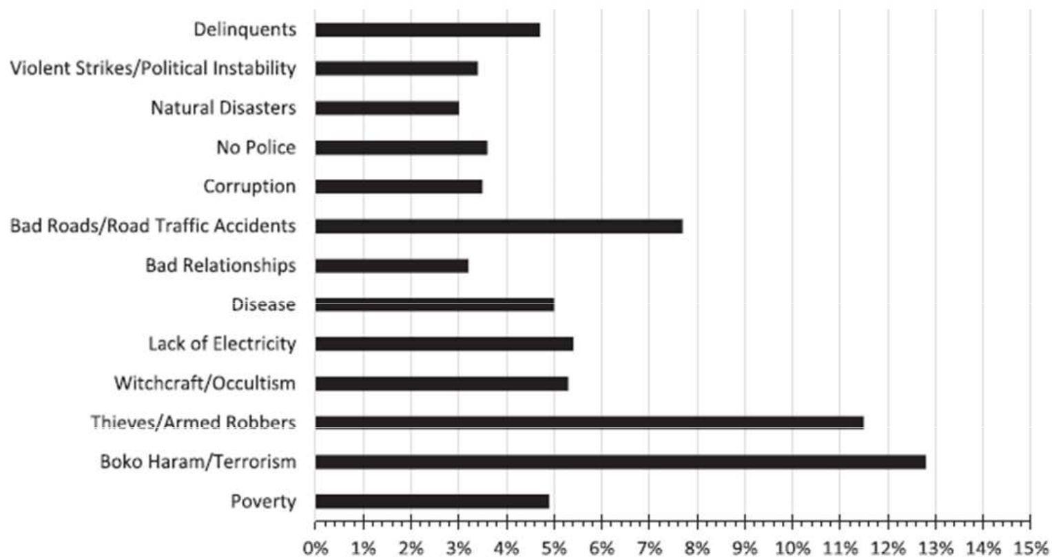
Security Threats
