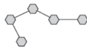
Chain network
