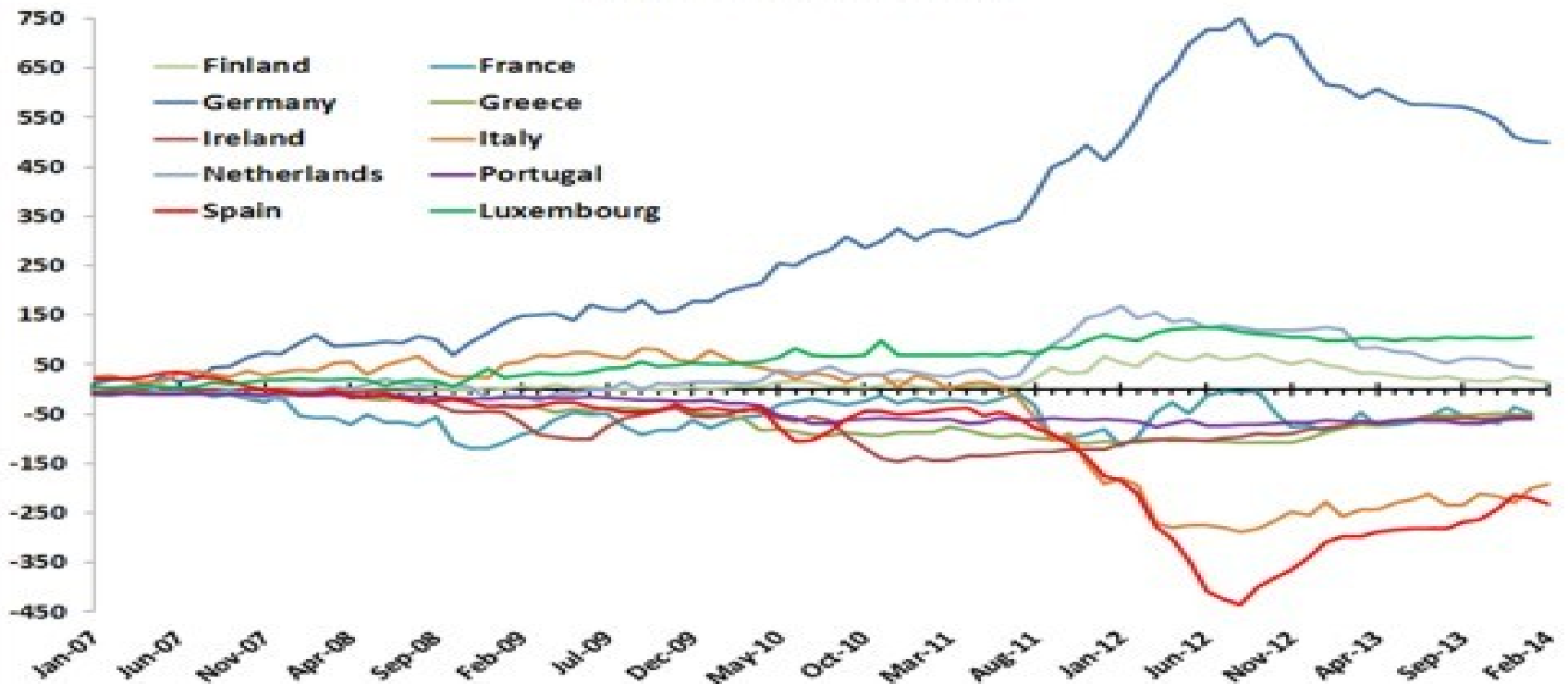
Target2-Balances [bn €]
