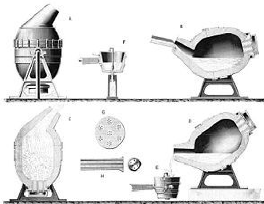
FIG. 65. THE FIRST PART OF BESSEMER'S CONVERTER AND LADLE.
