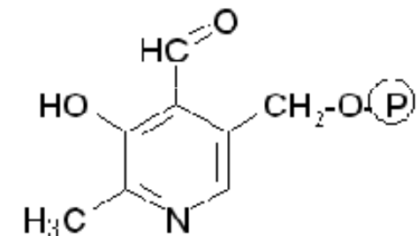
Pyridoxal phosphate (PLP)
