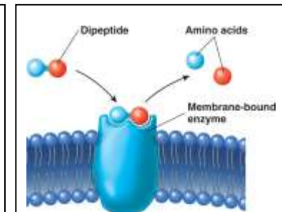
Enzymatic activity
