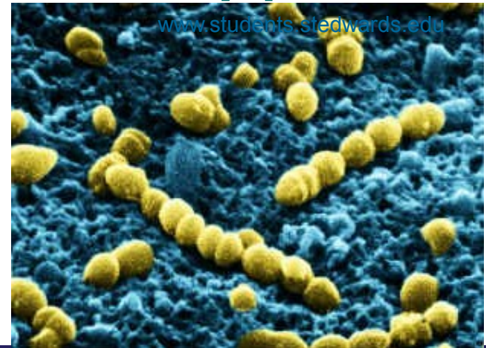
Figure 4. Cross-section of Streptococcus pneumoniae
