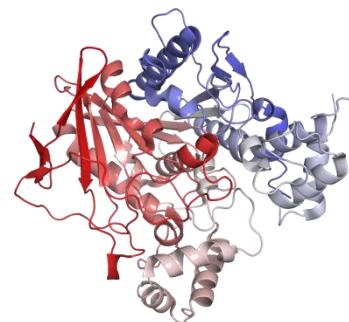
Acylcholinesteráza
