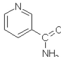
Nicotinamide
