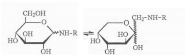
D-glukosylamin
