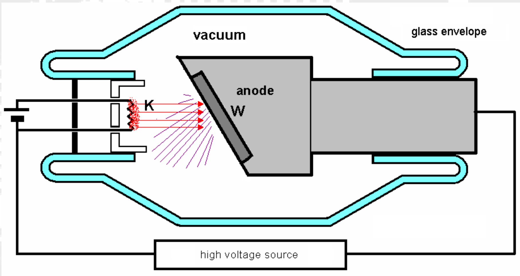
Scheme of an X-ray tube. K – hot filament cathode, W – tungsten plate. 6
