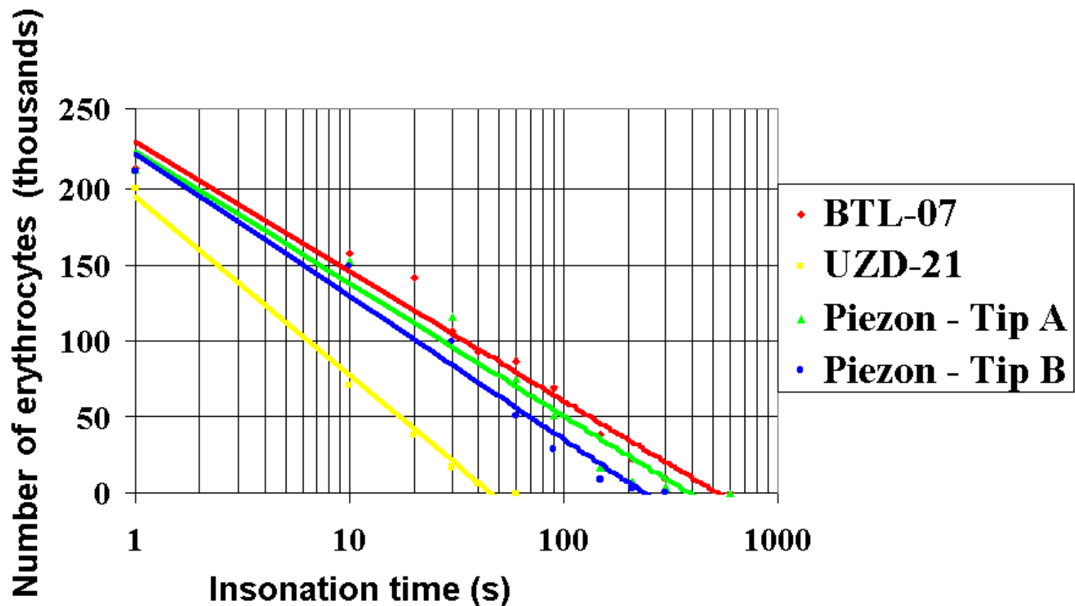
Comparison of cavitation effects in suspensions of erythrocytes
