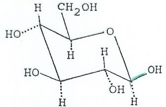
chair conformation of \beta -glucopyranose
