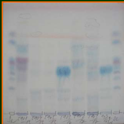
HPTLC – sacharidy
