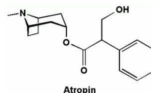
Atropin
