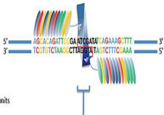
active FokI catalytic subunit heterodimer
