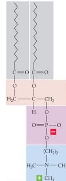
B DIPALMITOYL PHOSPHATIDYLCHOLINE (DPPC)
