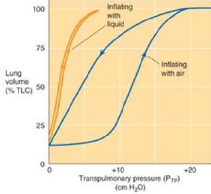
C DEFINITION OF SURFACE TENSION
