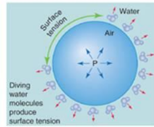
D SPHERICAL AIR-WATER INTERFACE
