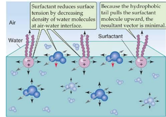
B DIPALMITOYL PHOSPHATIDYLCHOLINE (DPPC)
