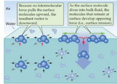
B FLAT AIR-WATER INTERFACE
