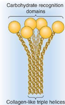
C THE SURFACTANT APOPROTEIN SP-A
