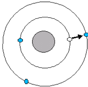
excitace
