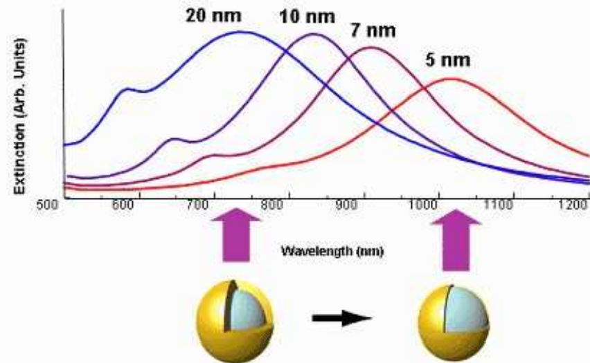
Thickness of the gold coating determines sensitivity of nanoshells to different wavelengths. The picture shows the results of theoretical calculations.
