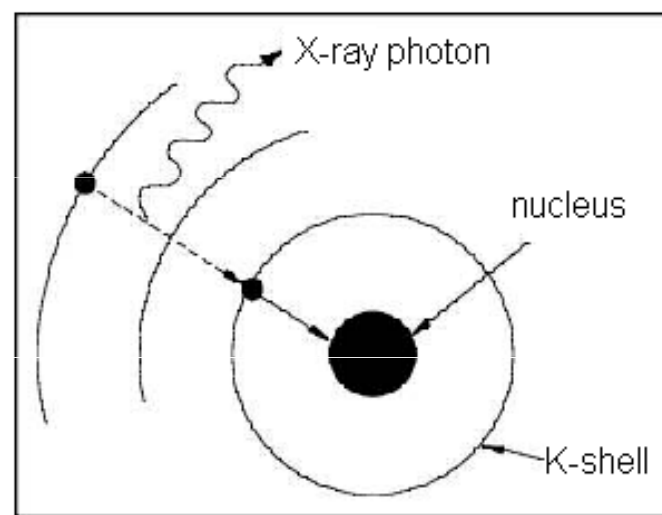
K-capture
