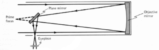
Newtonian telescopes
