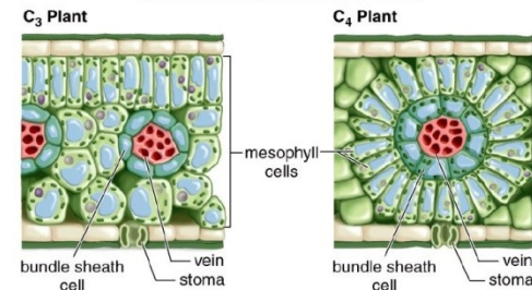
Chloroplast distribution in C 3 vs C 4 Plants
