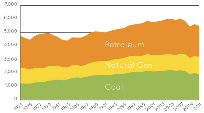
Carbon Dioxide Emissions from Fossil Fuels (million metric tons)
