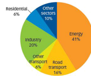
Figure 1. CO 2 emissions by sector
