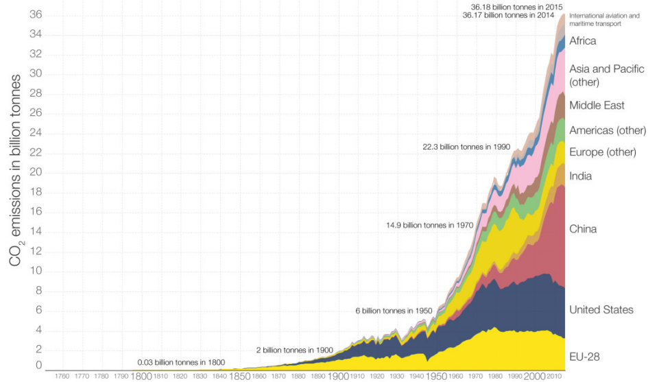
Global CO 2 emissions by world region, 1751 to 2015
