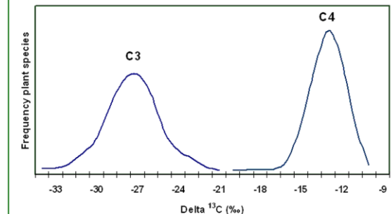
Distribution of \delta^{13}\text{C} among C 3 and C 4 plant species
