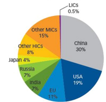
Figure 2. Energy-related CO 2 emissions by country
