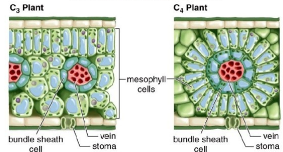
Chloroplast distribution in C 3 vs. C 4 Plants
