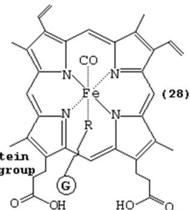
Carboxyhaemoglobin
