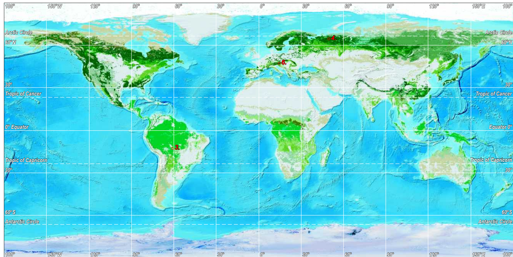
1. Global natural forest and shrub cover.
