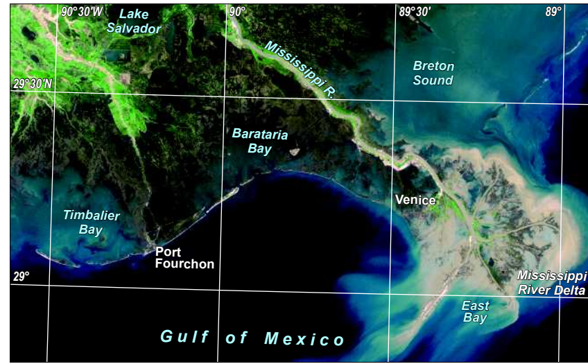
2a. Louisiana's coast line in 1976.
