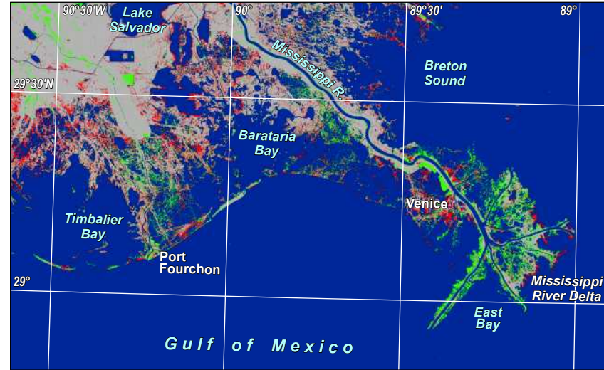
2b. Land shifting on Louisiana's coast line between 1976 and 2001.
