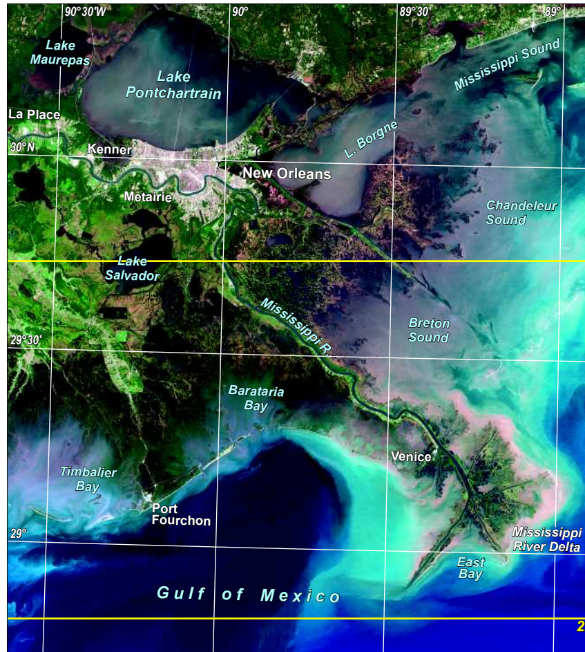
2a. Louisiana's coast line in 1976.
