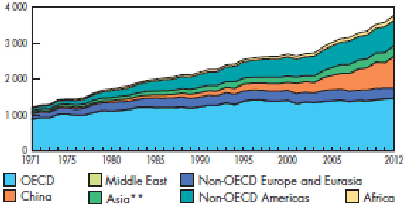
Hydro production* from 1971 to 2012 by region (TWh)
