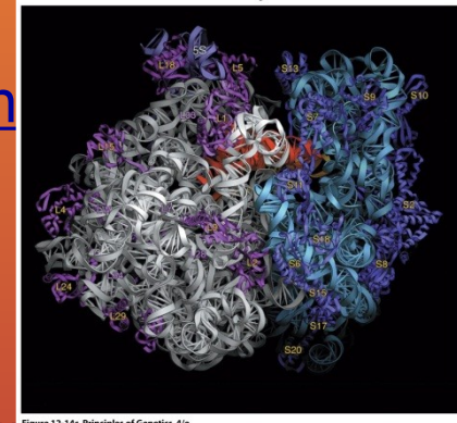
70S ribosome—crystal structure
