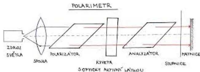
A Laurent Polarimeter
