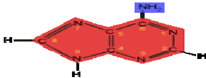
Adenin (A)
