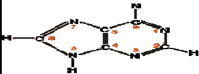
Purin
