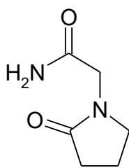
piracetam
