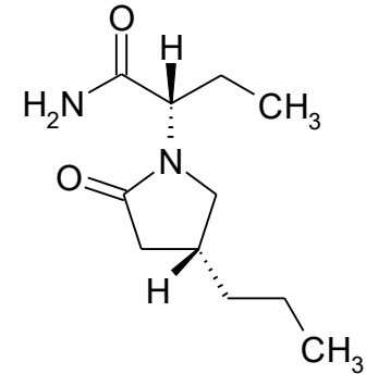
brivaracetam
