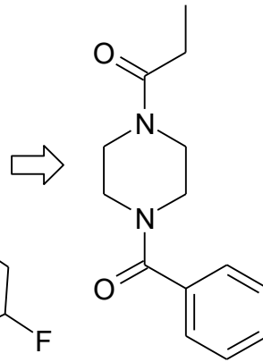
sunifiram
