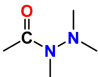
hydrazid
