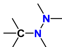
hydrazin
