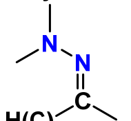
hydrazon
