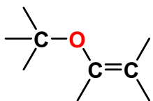
enol ether
