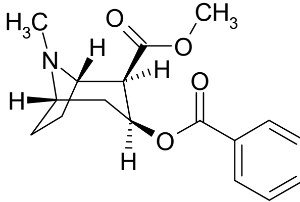
methyl-(1S,2R,3S,5S)-3-(benzoyloxy)-8-methyl-8-azabicyclo[3.2.1]oktan-2-karboxylát kokain
