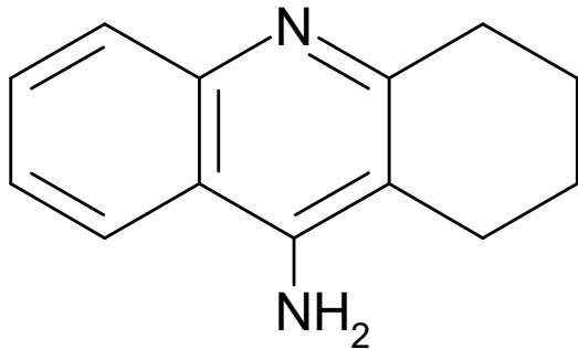
9-amino-1,2,3,4-tetrahydroakridin takrin
