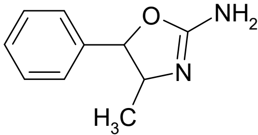
2-amino-5-fenyl-4-methyl-4,5-dihydro-1,3-oxazol
