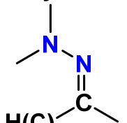
hydrazon
