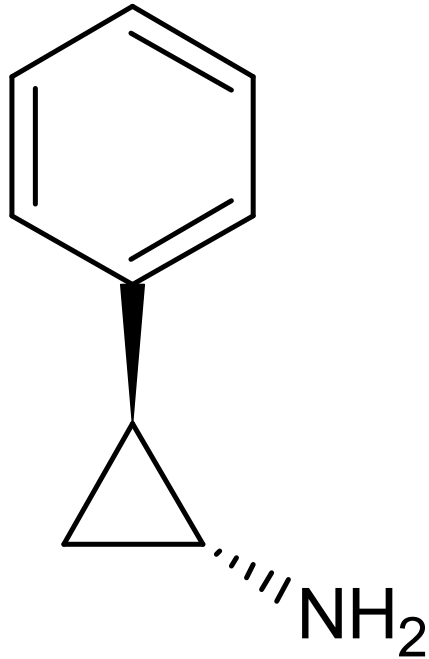
trans - 1-amino-2-phenylcyclopropane
