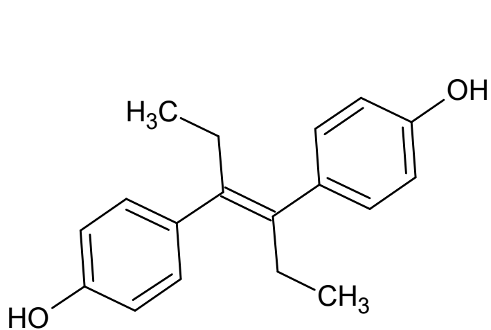
trans -diethylstilbestrol
