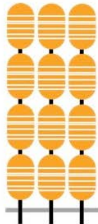
Receptory TNF
