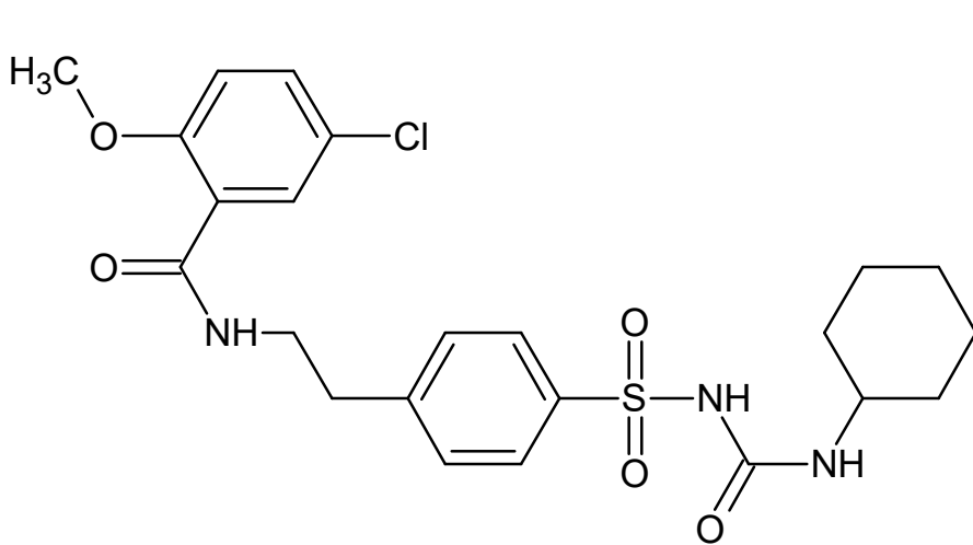
glibenclamide
