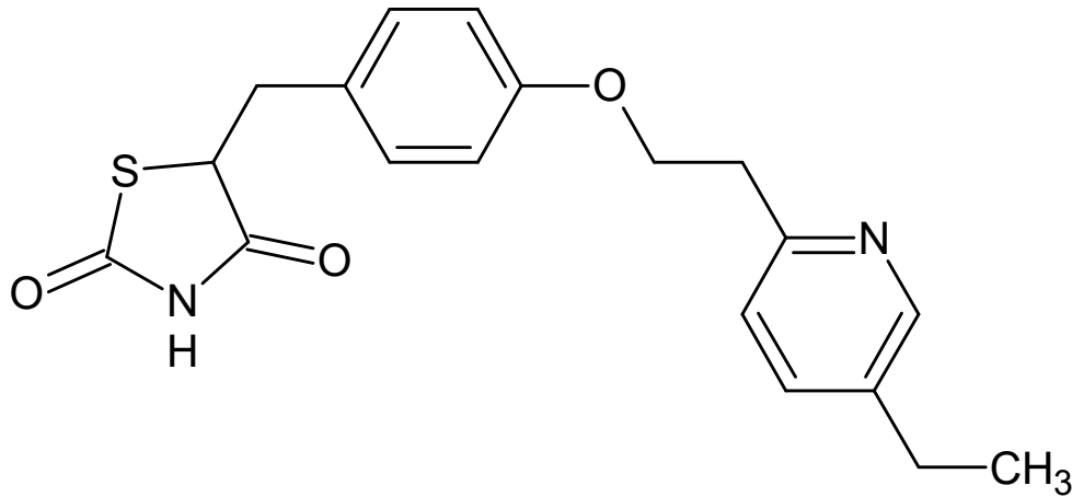
pioglitazone
