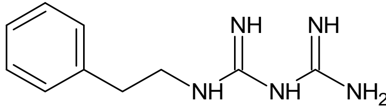
1-(2-phenylethyl)guanidine fenformin
