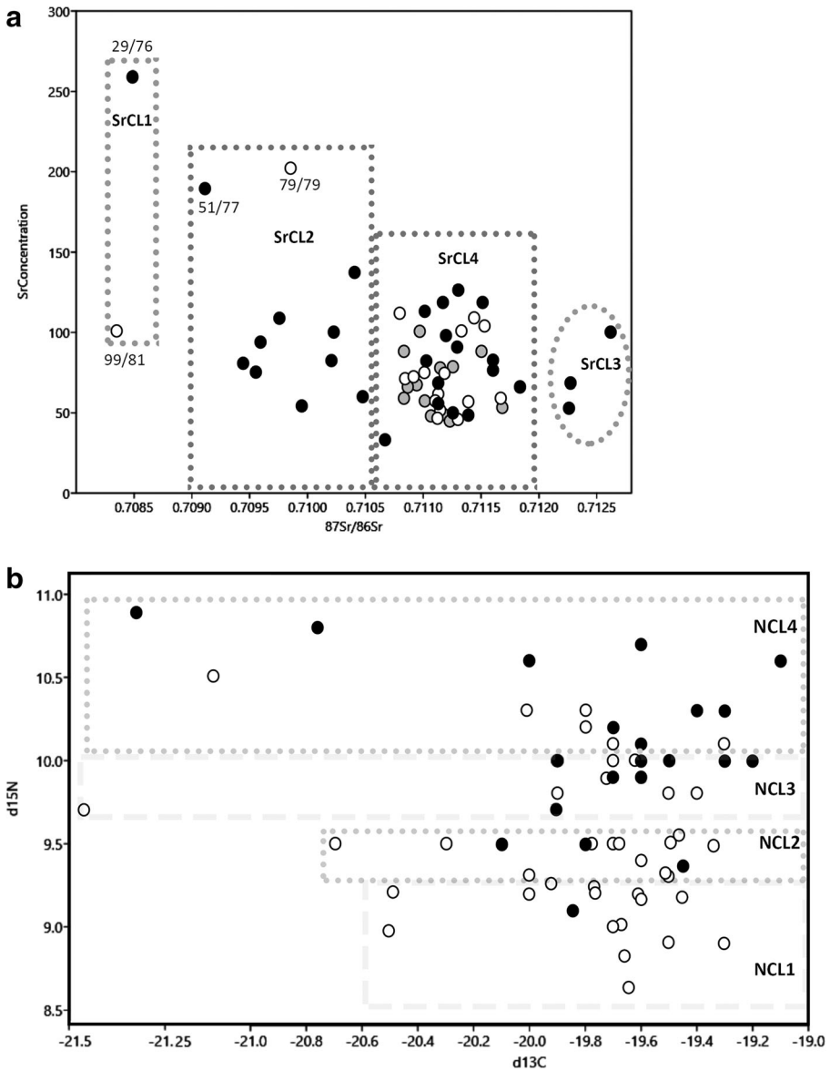
Fig. 11 a XY Biplot including ^{87}\text{Sr}/^{86}\text{Sr} values, ^{87}\text{Sr}/^{86}\text{Sr} concentration and strontium clusters 1–4. Black dots correspond to females, grey dots to non-adults and white dots to males. b XY Biplot including \delta^{15}\text{N} , \delta^{13}\text{C} isotope values and nitrogen clusters 1–4. Black dots correspond to males, white dots to female individuals
