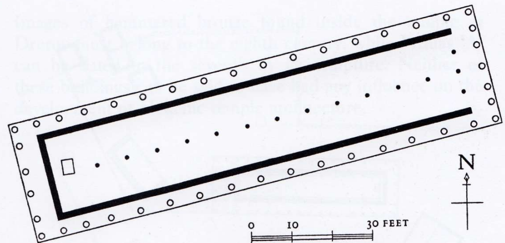
84. Samos, first Heraion, eighth century, restored plan
