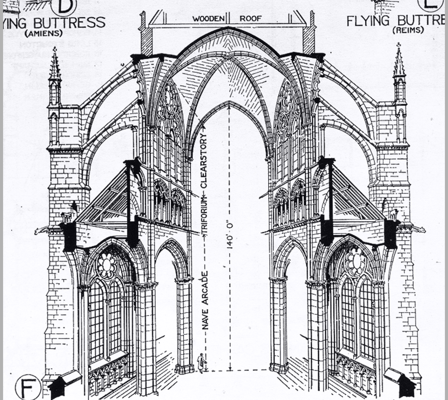
TRANSVERSE SECTION OF A TYPICAL GOTHIC CATHEDRAL (AMIENS)
