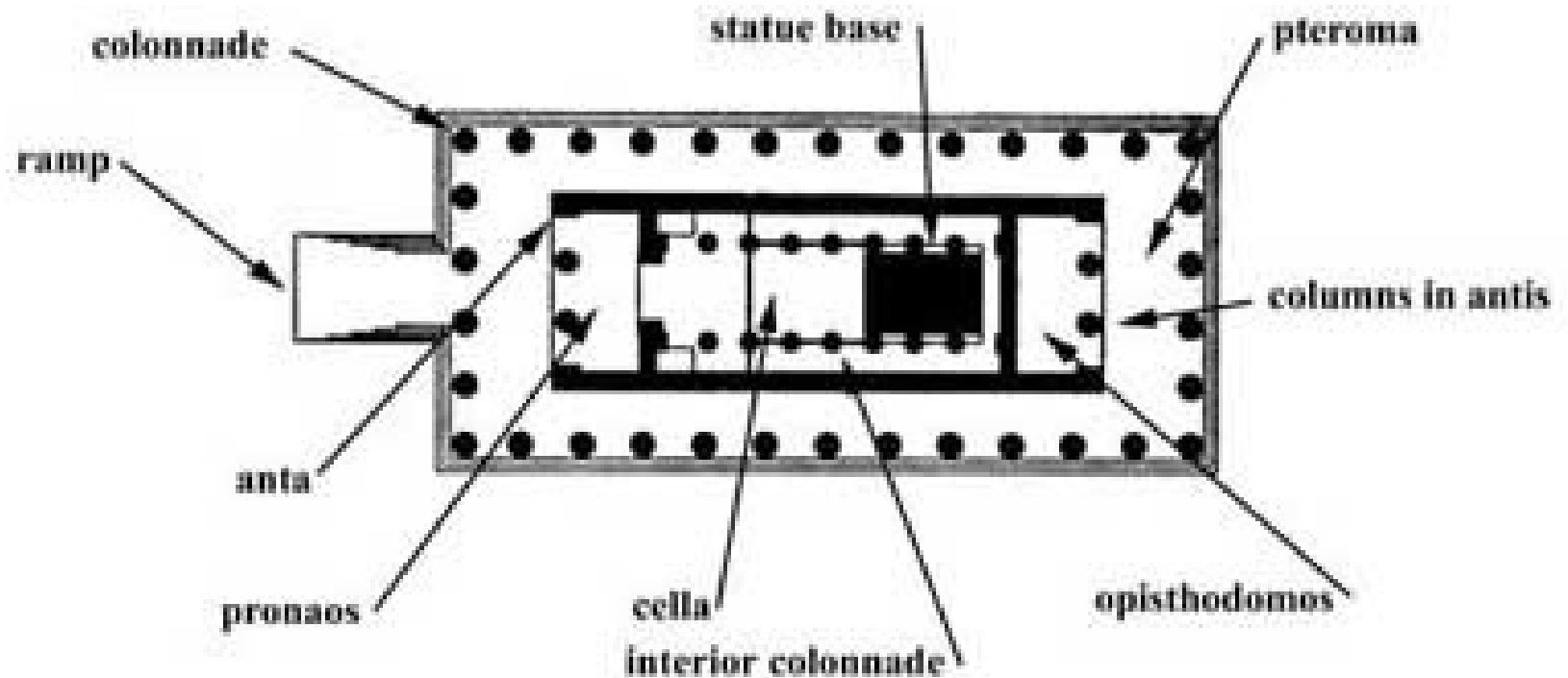
TEMPLE OF ZEUS AT OLYMPIA
