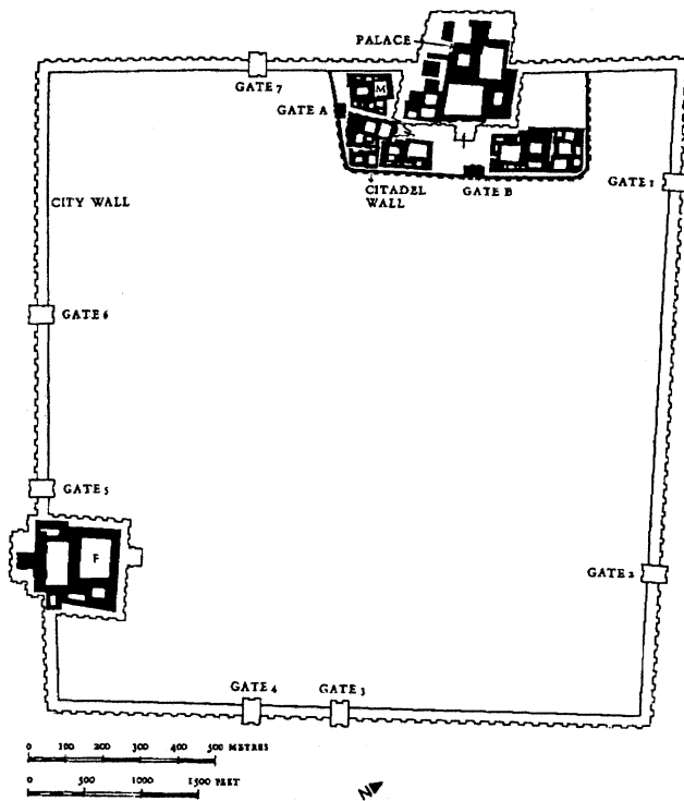
FIG. 5. Khorsabad. Plan of city walls with citadel, built by Sargon II, 8th century B.C. From Frankfort, Art and Architecture , fig. 165.
